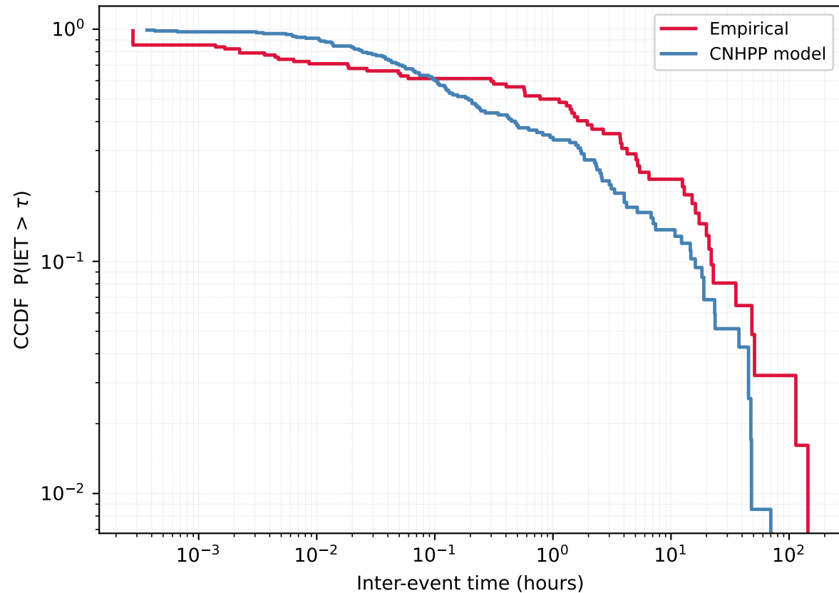
User 6938249017 - Empirical vs CNHPP model
